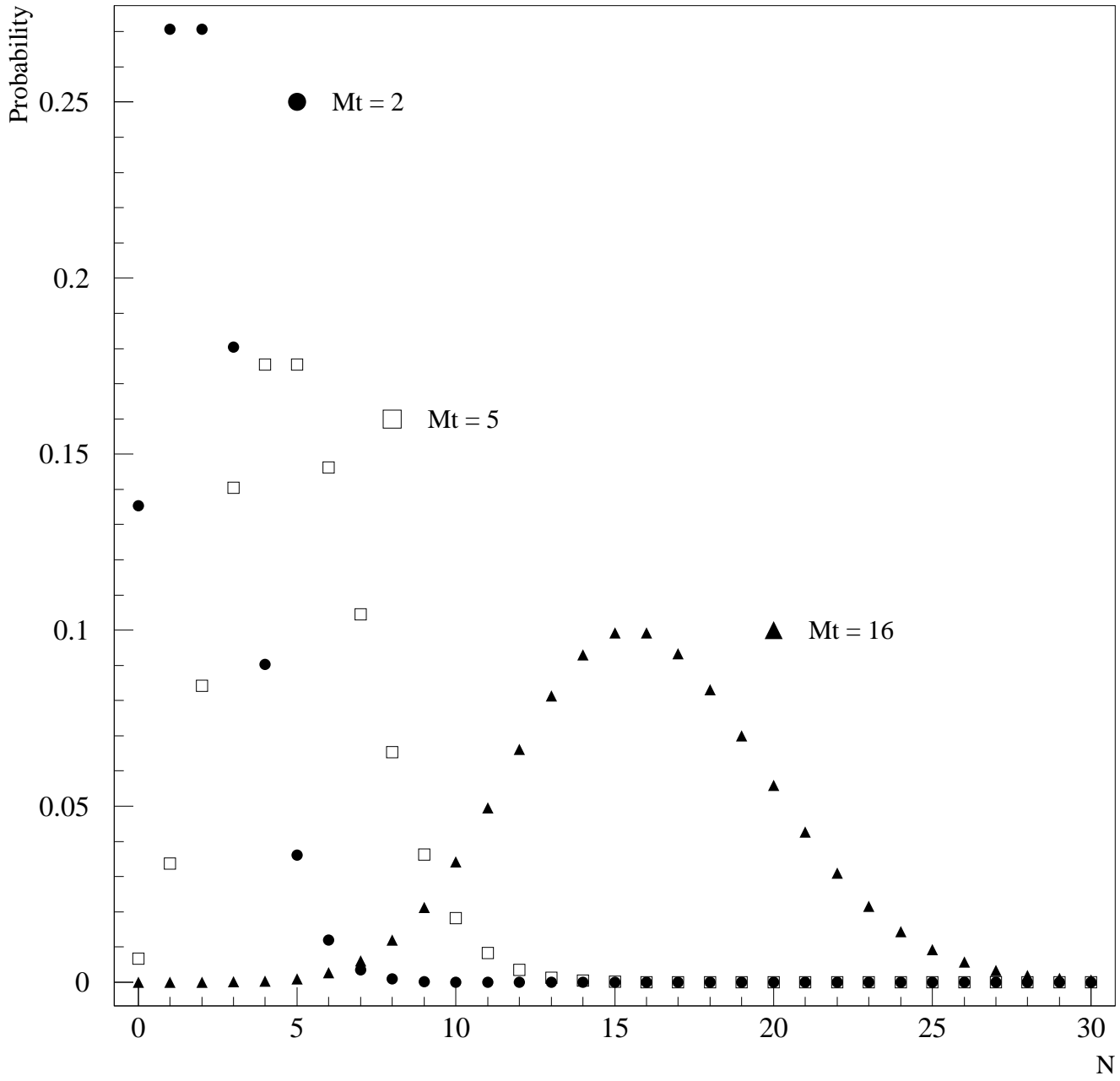
Poisson Distribution for Different values of Mt
