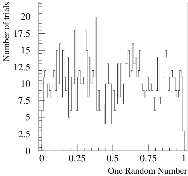
Summing Uniformly Distributed (0–1) Random Numbers
